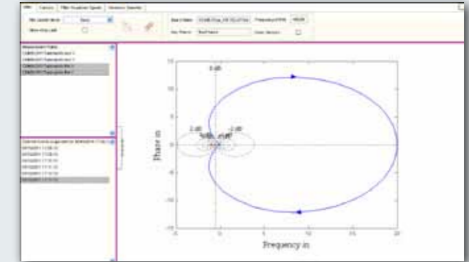
NYQUIST: Nyquist diagram for ramp-up / coast down analysis.
